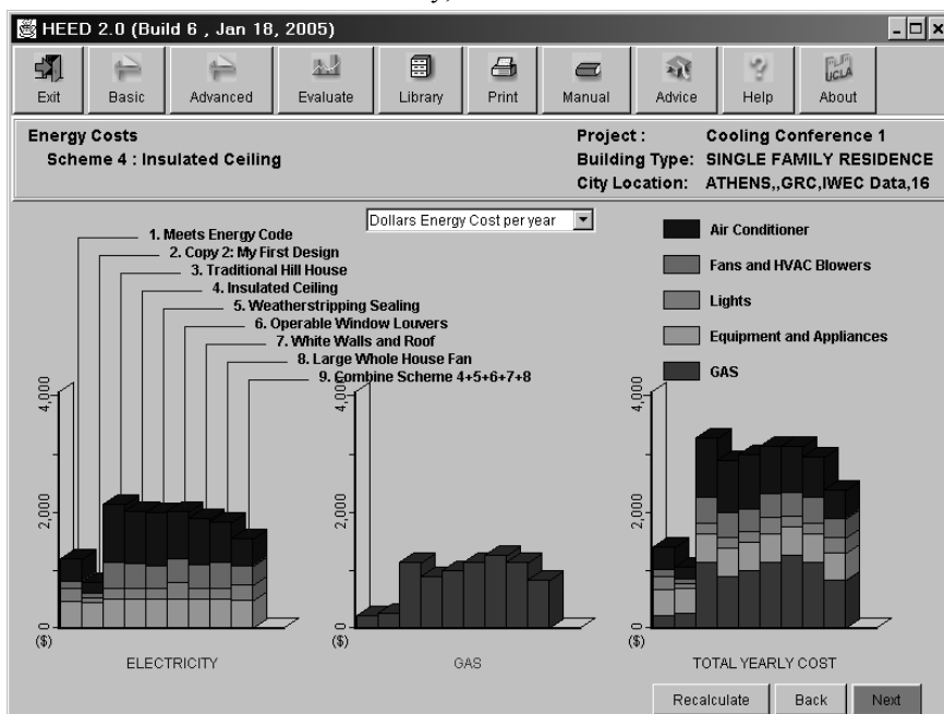
Figure 4: Energy Costs for all schemes are shown comparatively. Air Conditioning is the top (darkest) portion of the Electricity bars. Schemes 3 to 9 are organized in order of increasing cooling effectiveness. Notice that some good cooling strategies produce worse heating energy consumption.
