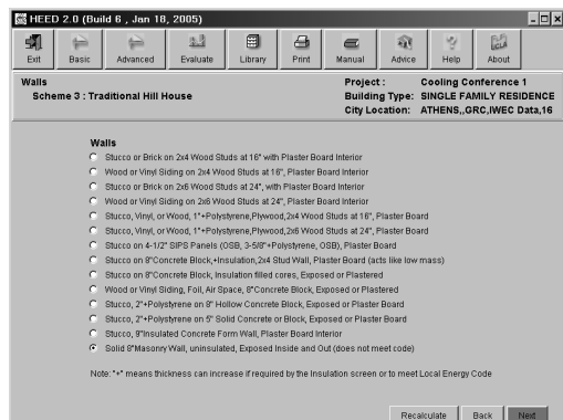
Figure 3: All aspects of building design and construction like Ventilation, Heating and Cooling Systems, Operable Shading, and Appliances can be defined by selecting from lists like this one.
