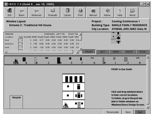
Figure 2: Window Layout: The user can click and drag windows from the catalog bar into the correct location to accurately compose each elevation, in this case the 4-story South elevation. Any of the green buttons can be clicked to show each of the other elevations or the roof.
