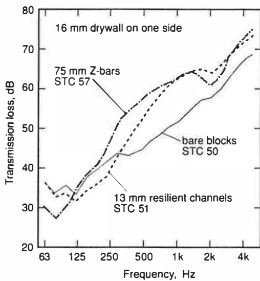
Figure 5 Sound transmission loss through different wall assemblies
