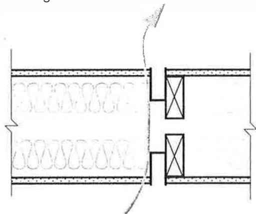
Figure 18 Leakage through electrical boxes
