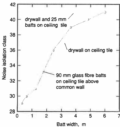
Figure 23 Noise isolation class achieved by plenum/ceiling treatment
