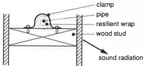
Figure 12 Plumbing noise test set-up
