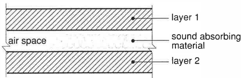
Figure 3 Idealized wall section
