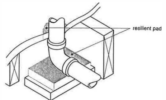
Figure 10 Possible means of isolating plumbing from sound-conducting elements
