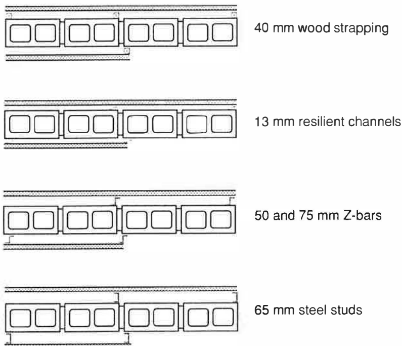
Figure 4 Wall assemblies tested for sound transmission loss
