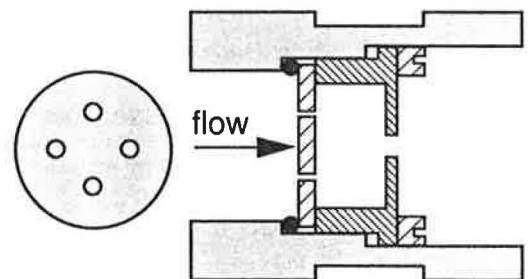
Figure 11 Cross section through the standard noise source
