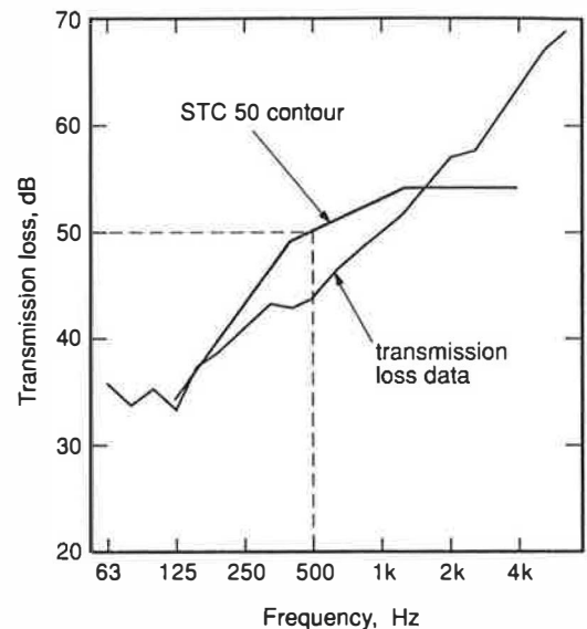
Figure 2 STC contour fitted to TL curve for concrete block
