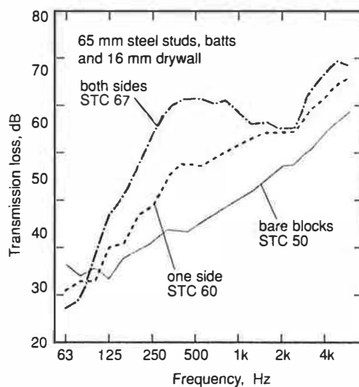
Figure 8 Poor transmission loss performance (low mass-air-mass resonance) below 125 Hz does not affect the STC rating
