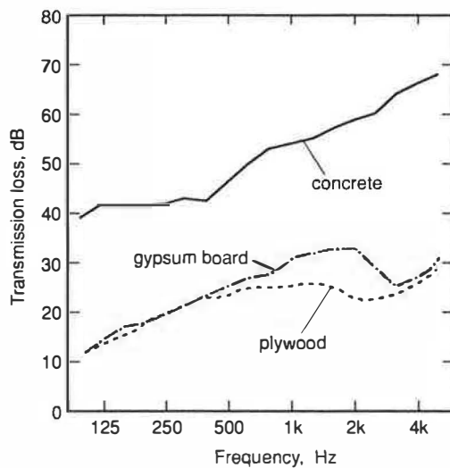
Figure 1 Sound transmission loss through building materials
