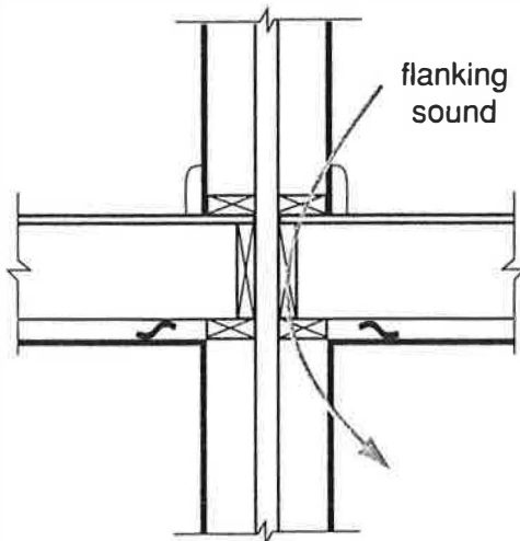
Figure 16 Sound flanking vertically through walls
