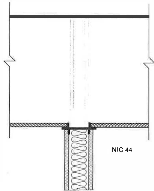
Figure 24 Wall construction extended through plenum space
