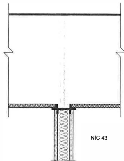
Figure 25 Blocking panels carried through plenum space
