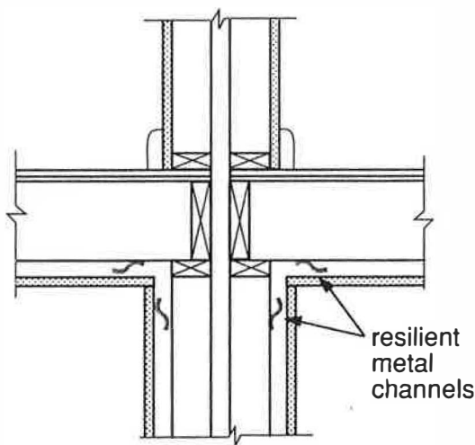
Figure 17 Resilient channels used to reduce flanking noise
