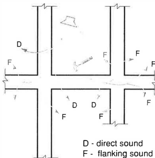
Figure 14 Flanking sound through building construction
