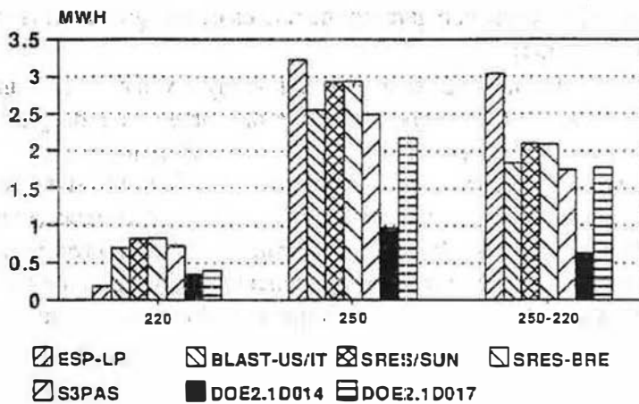
Figure 4. IEA BESTEST Exterior Shortwave Absorptance Effect (Cases 220,250) Annual Cooling Loads Indicating Discovered DOE-2.1D Disagreement
