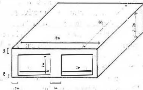
Figure 1. IEA BESTEST Base Building with Unshaded South Facing Windows
