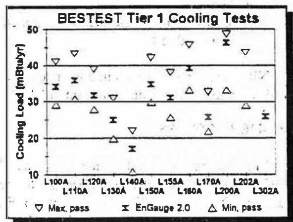
Figure 9. Comparison of Cooling Loads for EnGauge 2.0 versus HERS BESTEST Results Using Example Range Setting Criteria for Revised Raised-Wood-Floor Coefficients by FSEC.
