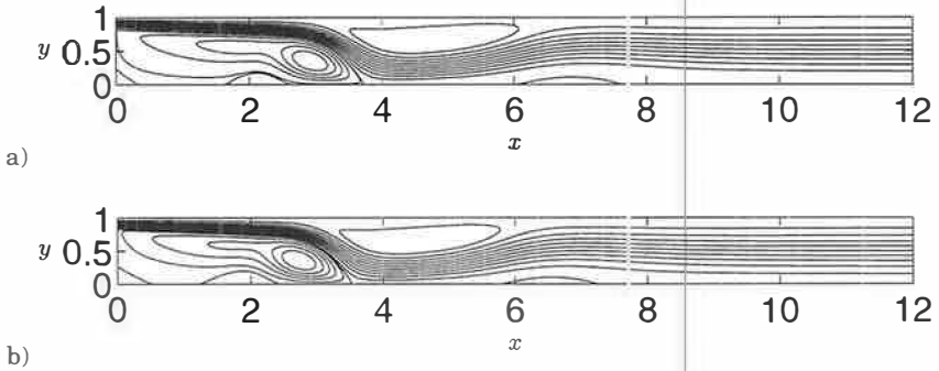
Figure 9: Contours of stream function. Re = 118 , h/H = 1/6 , Hybrid scheme, 160 \times 84 cells. a) Prescribed inlet profiles according to experiments (see Fig. 8 a). b) Parabolic inlet profile (see Fig. 3 b).
