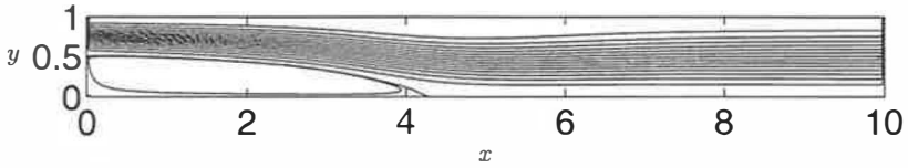
Figure 3: Contours of stream function. Re = 195 . h/H = 0.516
