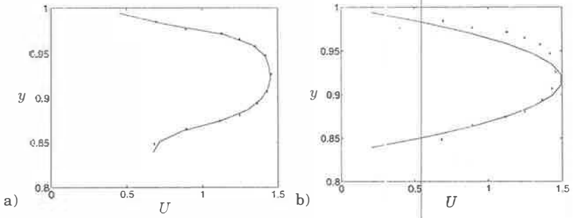
Figure 8: Inlet profiles. Solid lines: prescribed inlet U profiles in the predictions; markers: experiments. Re = 118 . h/H = 1/6 . 160 \times 84 cells. a) Interpolated profile from experiments. b) Parabolic profile.
