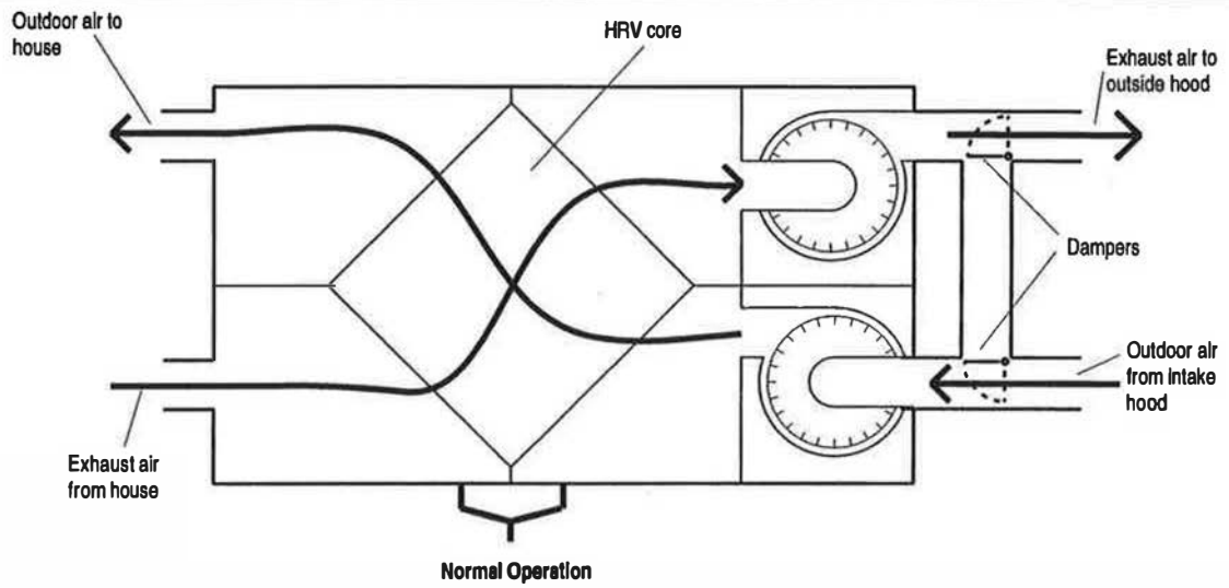
Figure 44: Other HRV Defrost Methods
