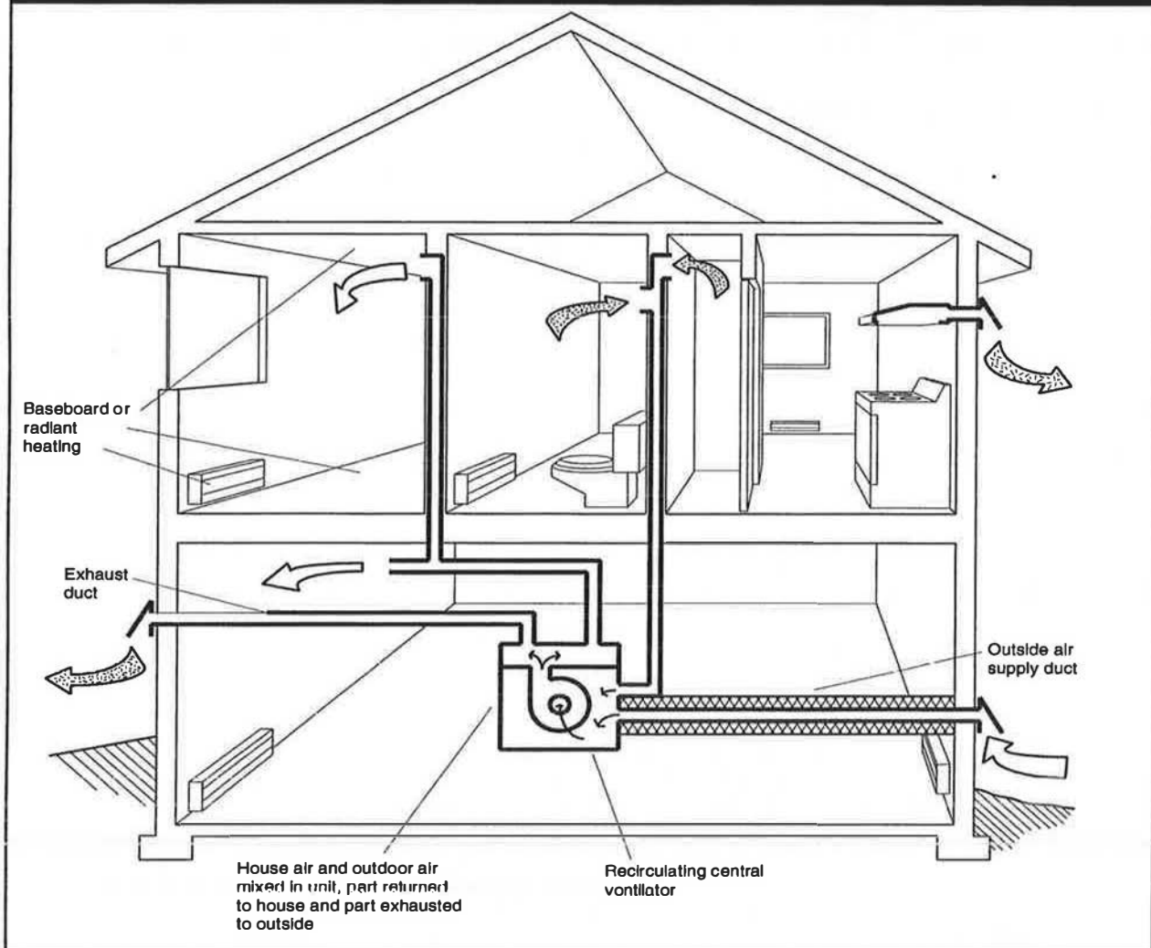
Figure 36: Recirculating Central Ventilation System
