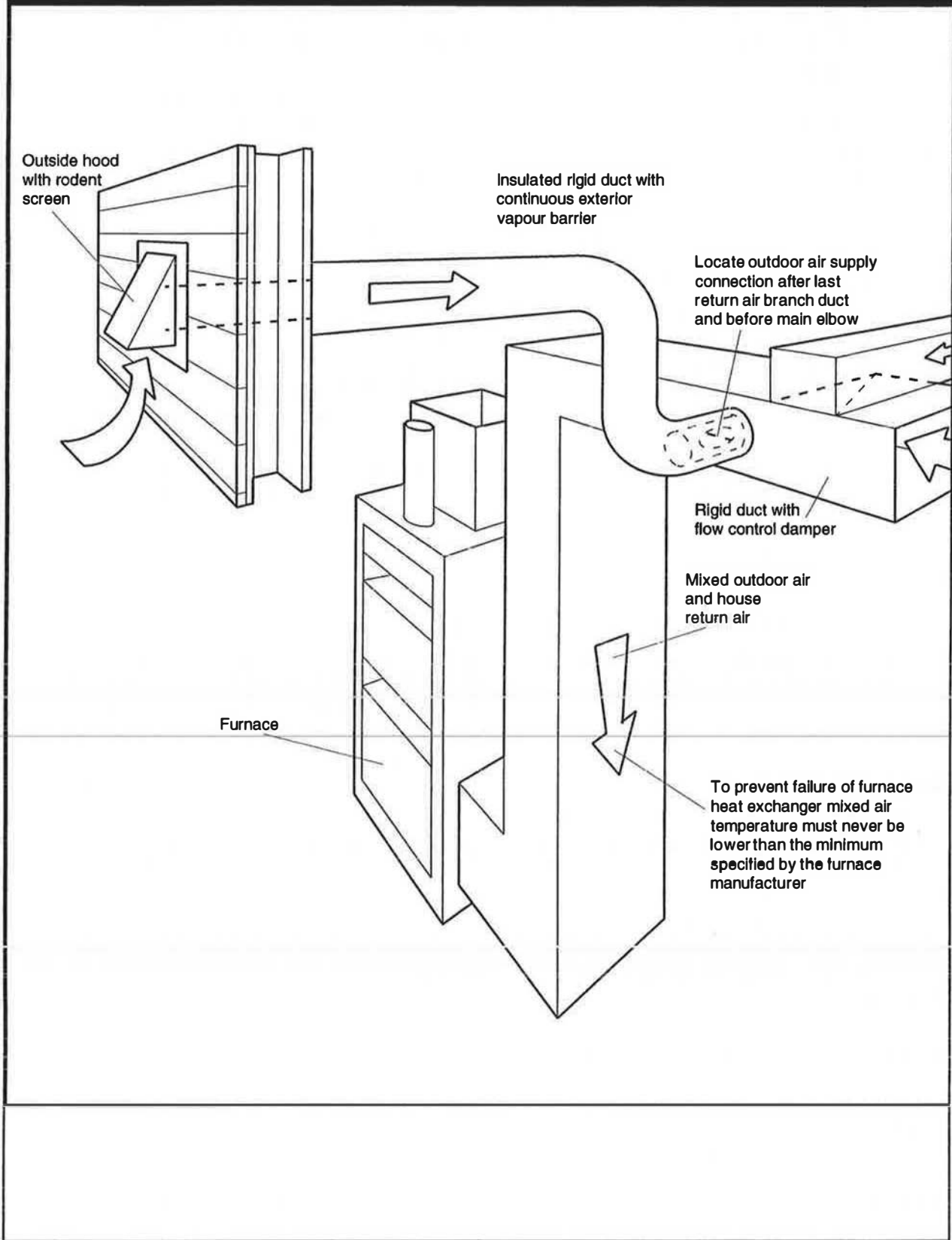
Figure 45: Built-Up Air Handler to Replace Furnace
