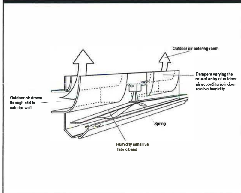
Figure 35: Humidity-Actuated Through Wall Supply
