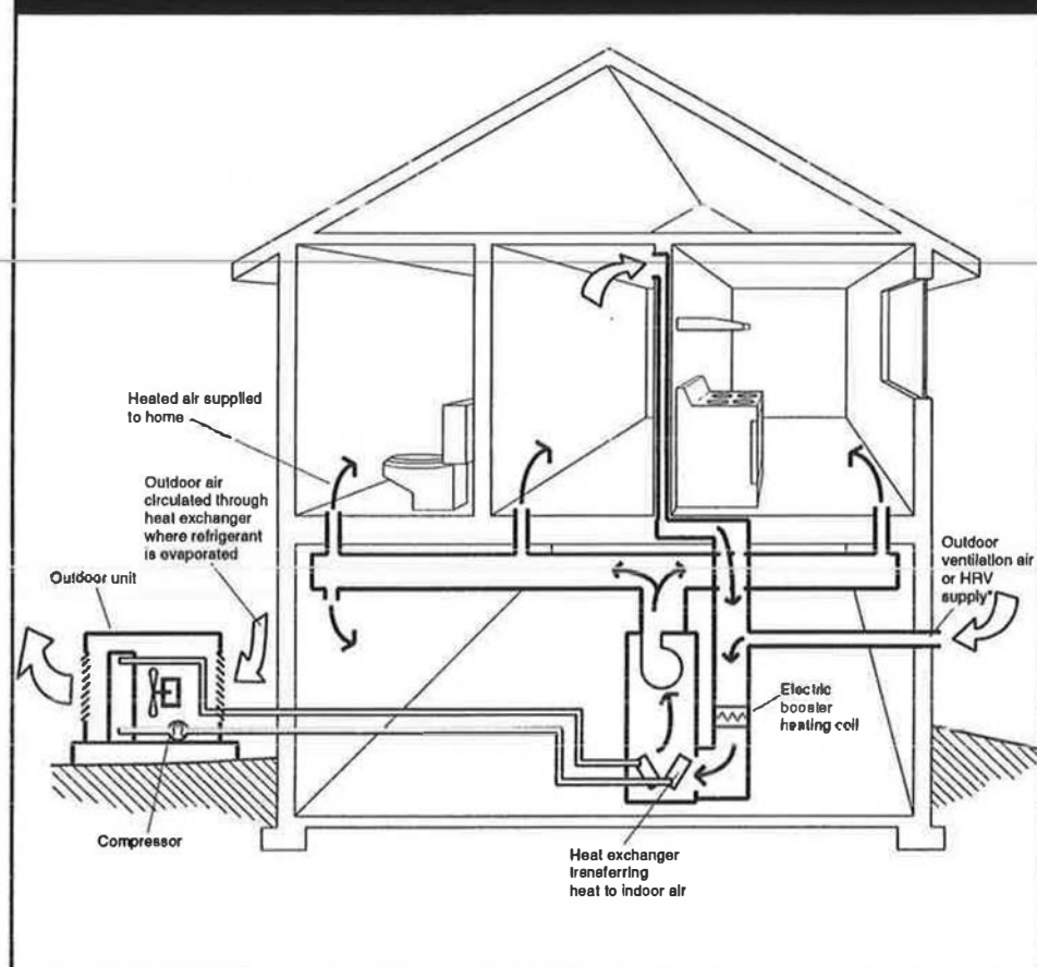
Figure 11: Air Source Heat Pump
