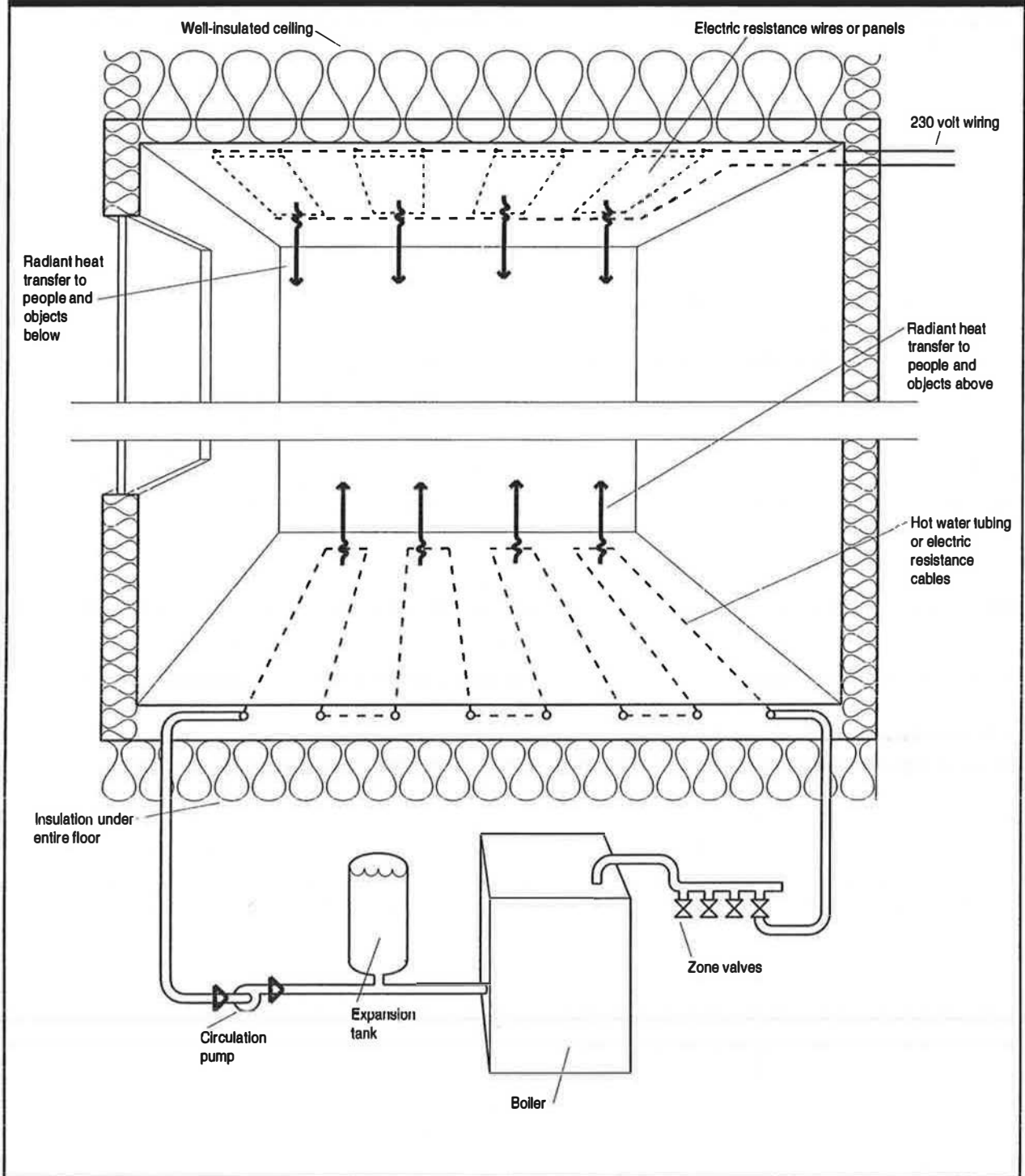
Figure 15: Radiant Heating
