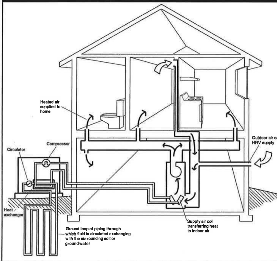
Figure 12: Ground Source Heat Pump
