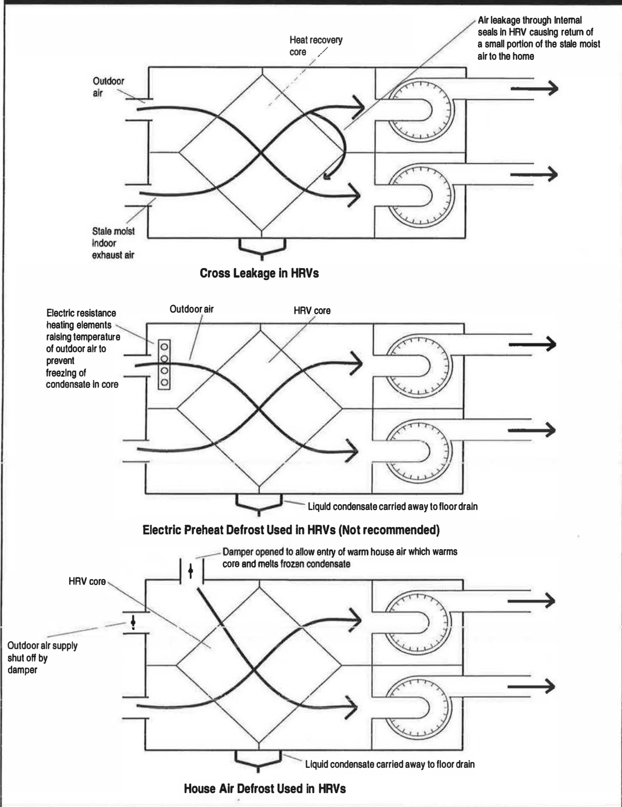
Figure 43: Cross-Leakage and Defrost Methods in HRVs
