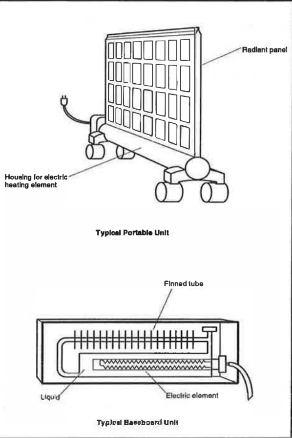
Figure 13: Baseboard Convection Heater
