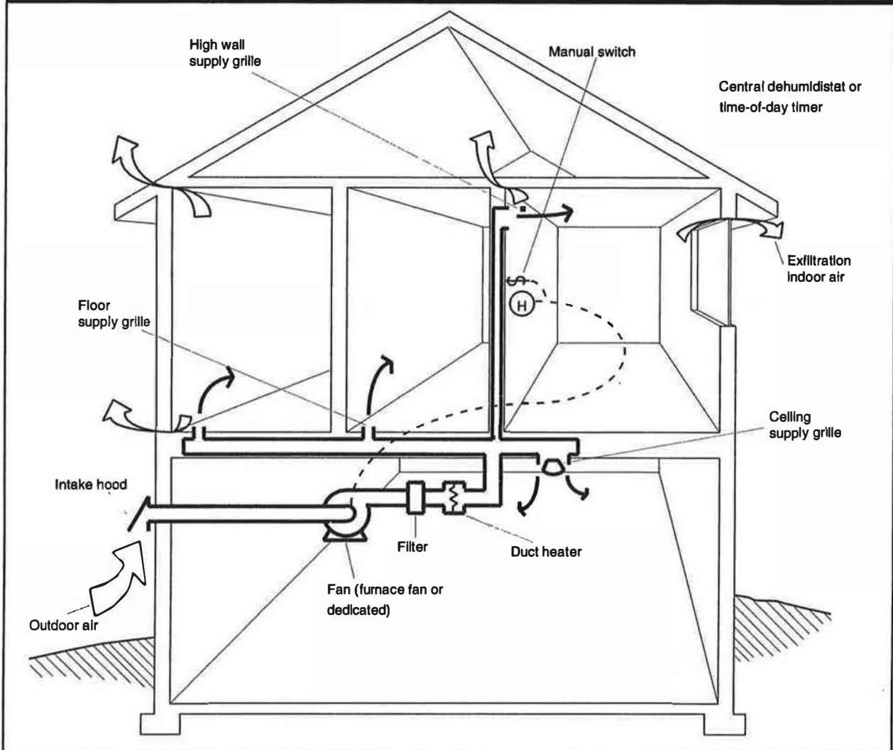
Figure 28: Ventilation—Supply Only
