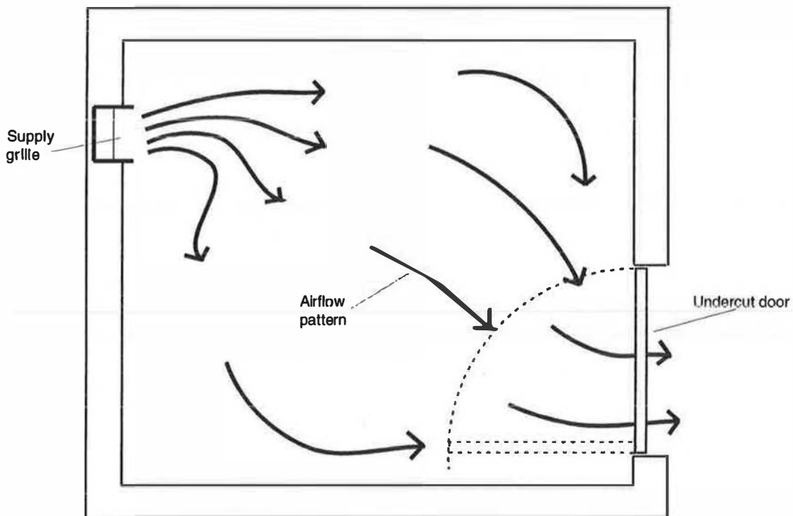
Plan View of Room
