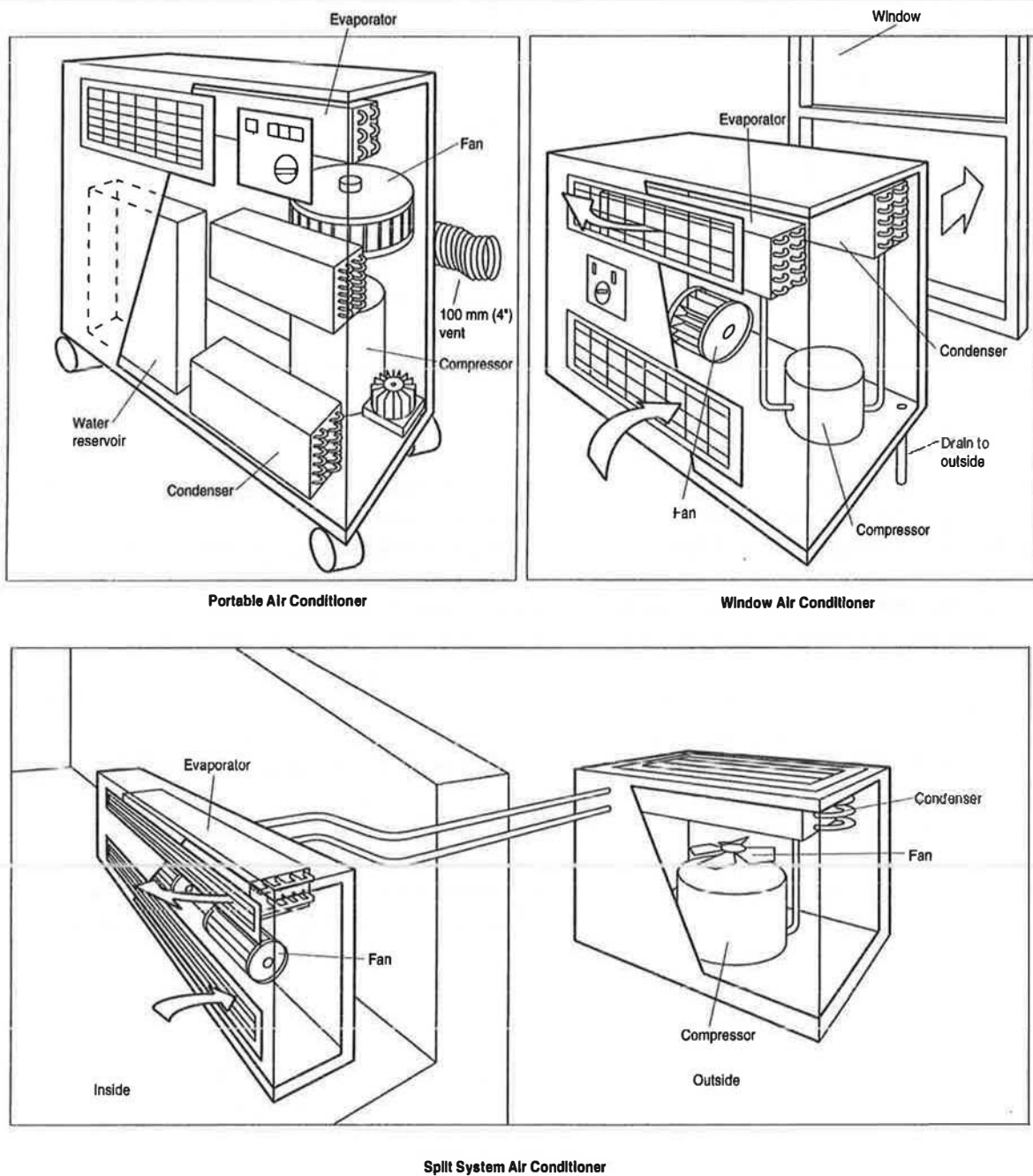
Figure 17: Compact Air Conditioners
