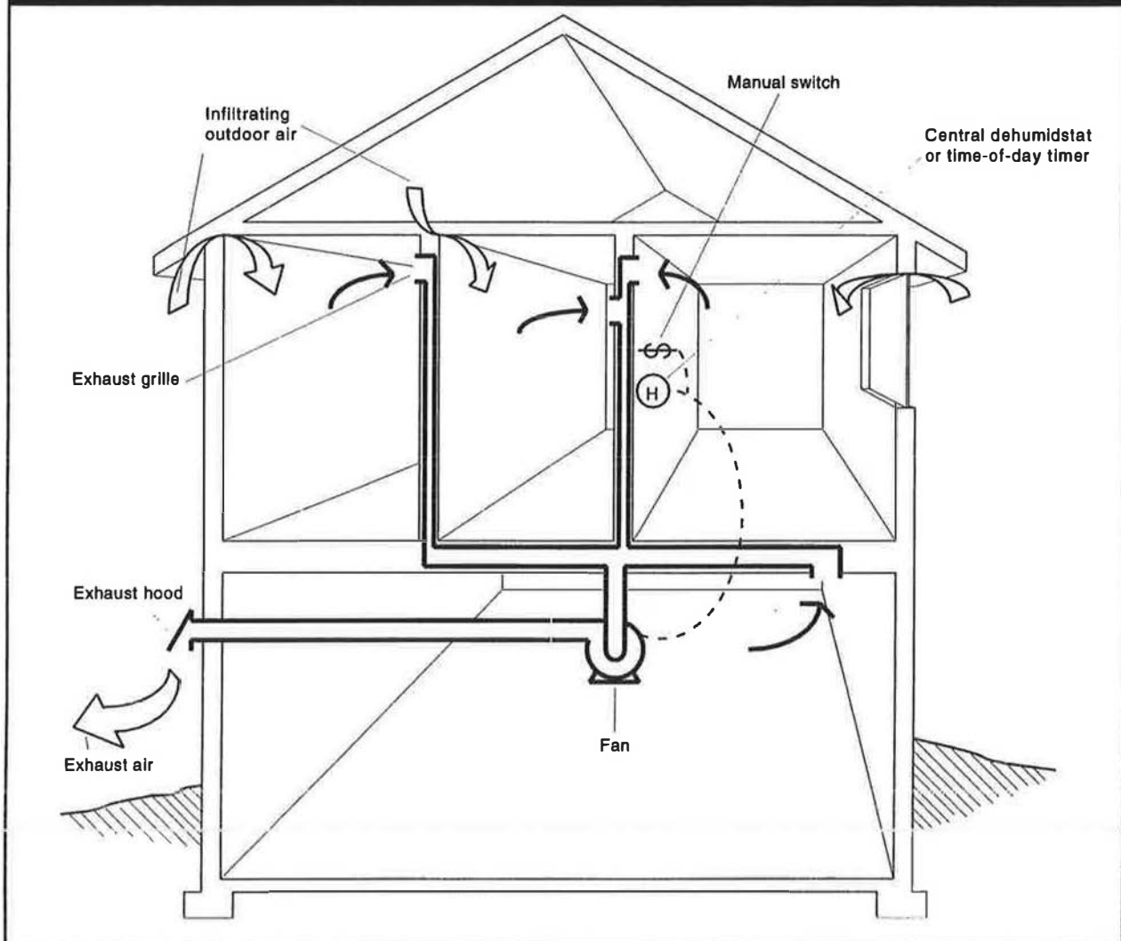
Figure 29: Ventilation—Exhaust Only
