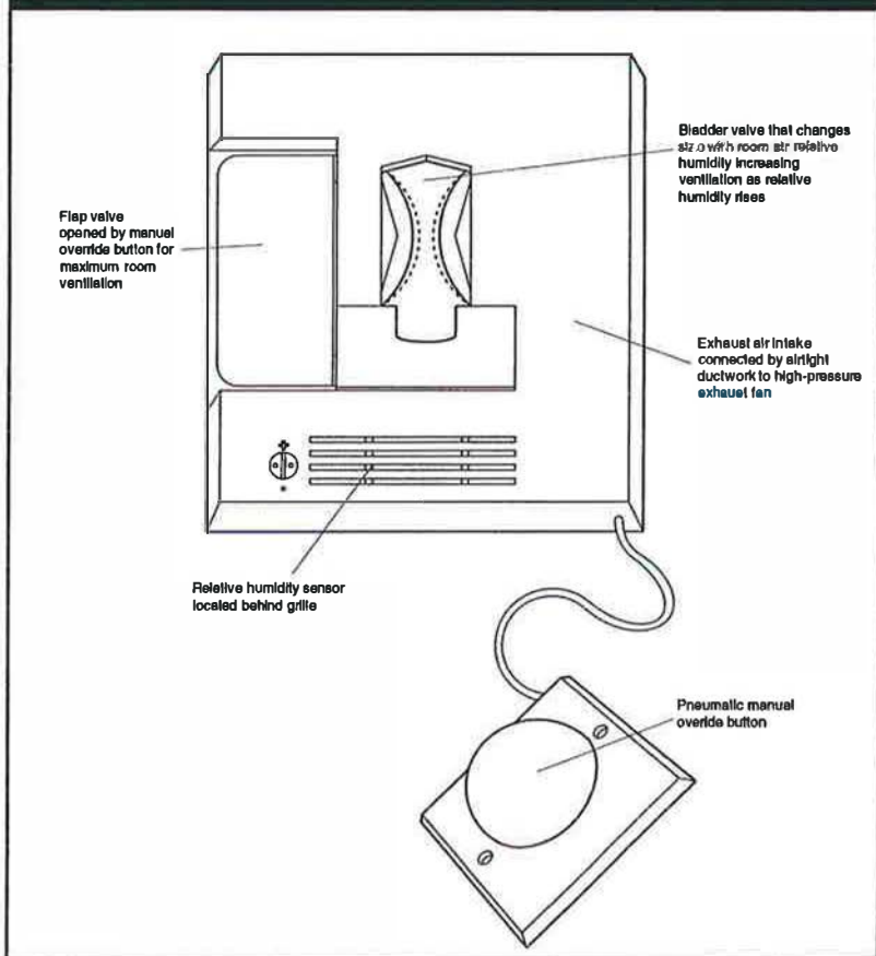
Figure 35: Humidity-Actuated Through Wall Supply
