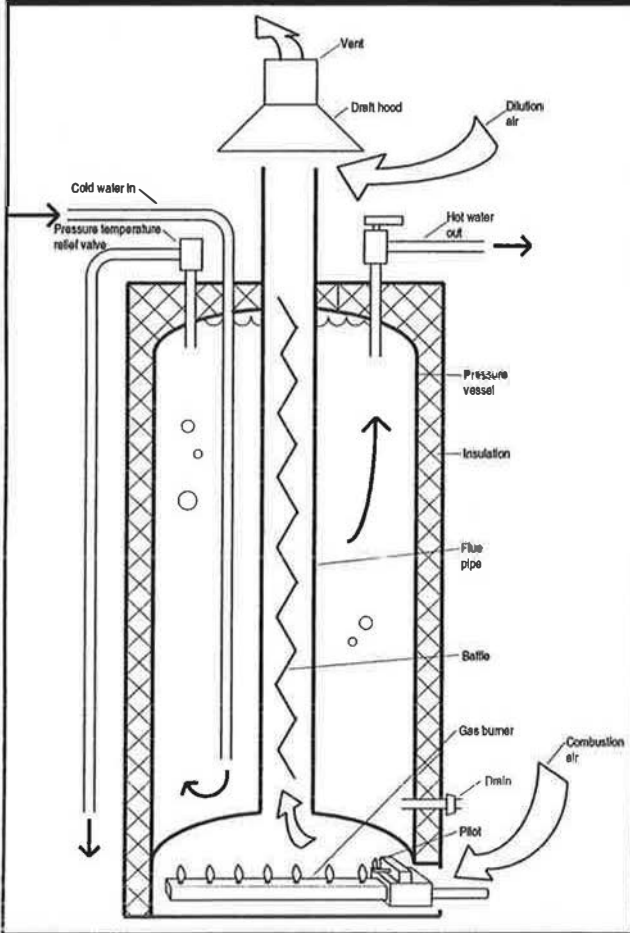
Figure 23: Naturally Aspirated Gas Hot Water Tank
