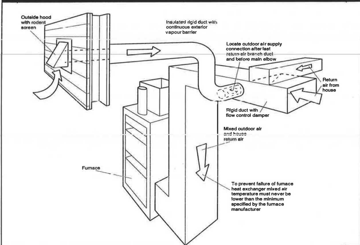
Figure 46: Outside Air Connection
