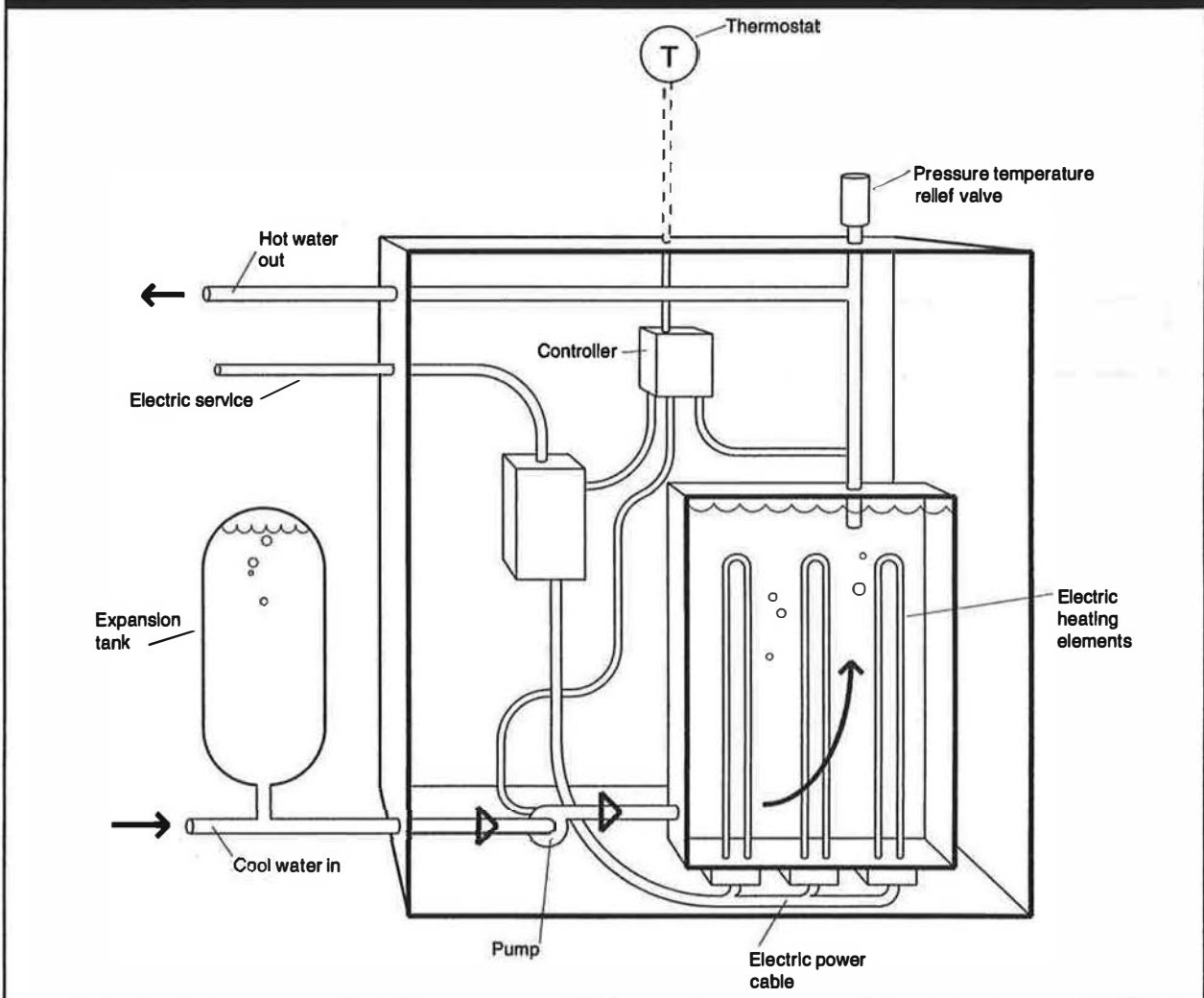
Figure 18: Typical Electric Boiler
