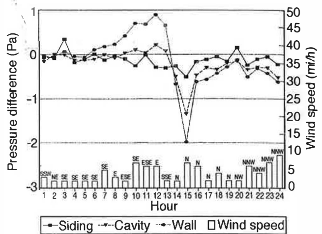
Figure 6 Hourly average pressure difference across the siding, between the outside and the cavity and across the entire wall, for wall OSEd, with hourly wind speed (10-minute average) and direction on October 18, 1996. Positive values indicate that the air pressure is infiltrative.
