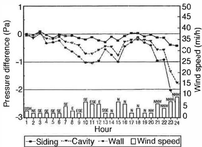
Figure 5 Hourly average pressure difference across the siding, between the outside and the cavity and across the entire wall, for wall OSWa, with hourly wind speed (10-minute average) and direction on October 18, 1996. Positive values indicate that the air pressure is infiltrative.
