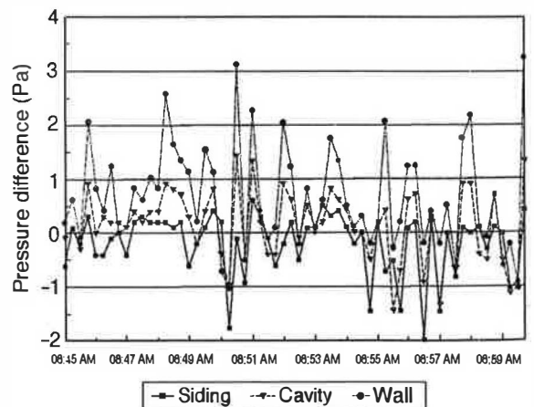
Figure 8 Instantaneous pressure difference (15-second sampling rate) across the siding, between the outside and the cavity, and across the entire wall for wall OSEd between 8:45 a.m. and 9:00 a.m. on October 18, 1996. Winds were from the southeast. Positive values indicate that the air pressure is infiltrative.
