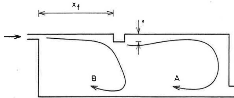
Fig. 6. Different steady state solutions for the three-dimensional flow pattern under isothermal conditions. Flow of type A is obtained for heights of the obstacle smaller than a critical value f_c .
