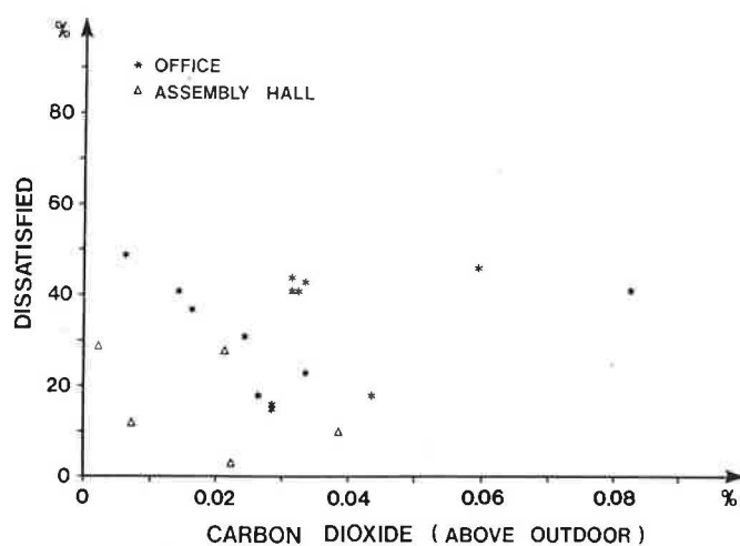
Fig. 3. Percentage of dissatisfied as a function of the carbon dioxide concentration above outdoor level (for the 20 occupied spaces).
