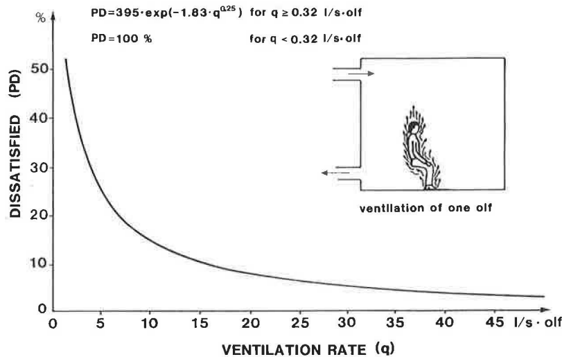
Fig. 7. The curve defines the percentage of dissatisfied persons caused by one standard person (one olf), when ventilated by unpolluted outdoor air at different ventilation rates [3].
