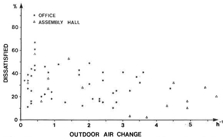
Fig. 2. Percentage of dissatisfied as a function of the outdoor air change.
