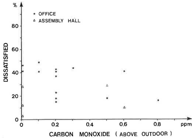
Fig. 4. Percentage of dissatisfied as a function of the carbon monoxide concentration above outdoor level (for the 20 occupied spaces).
