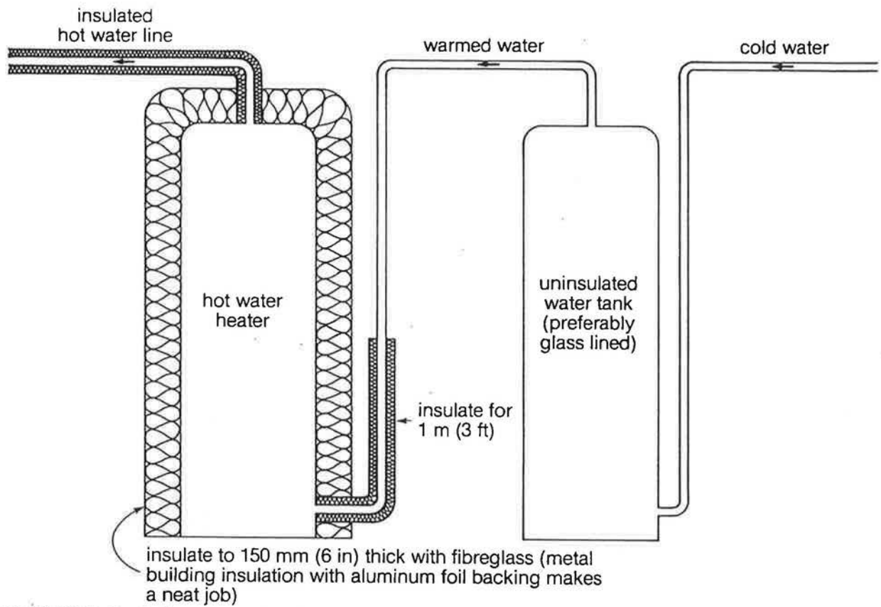
FIGURE 30. Technique for preheating hot water and insulating hot water tank
