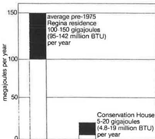
FIGURE 1. Annual space heating energy requirements
