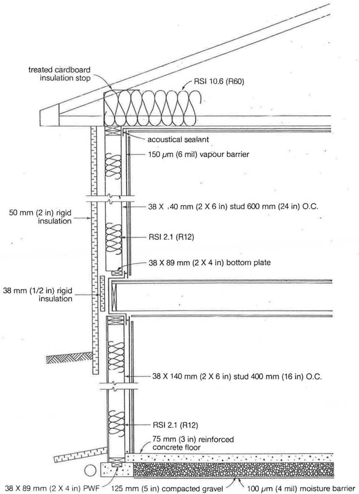
FIGURE 21. Wall section
