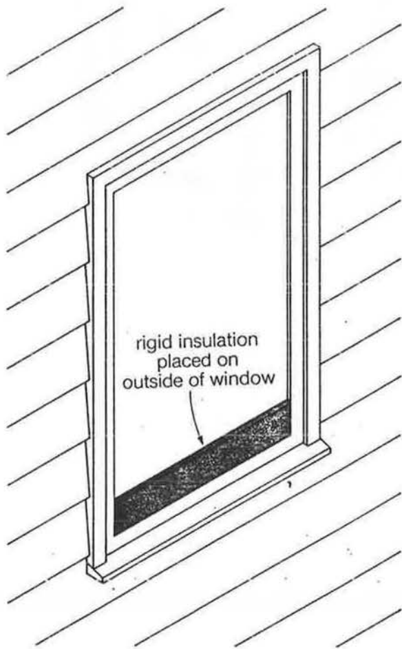
FIGURE 16. Technique for reducing condensation at the bottom of windows
