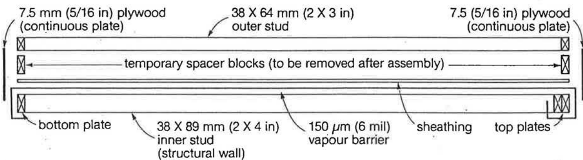
FIGURE 10. Double stud wall assembly
