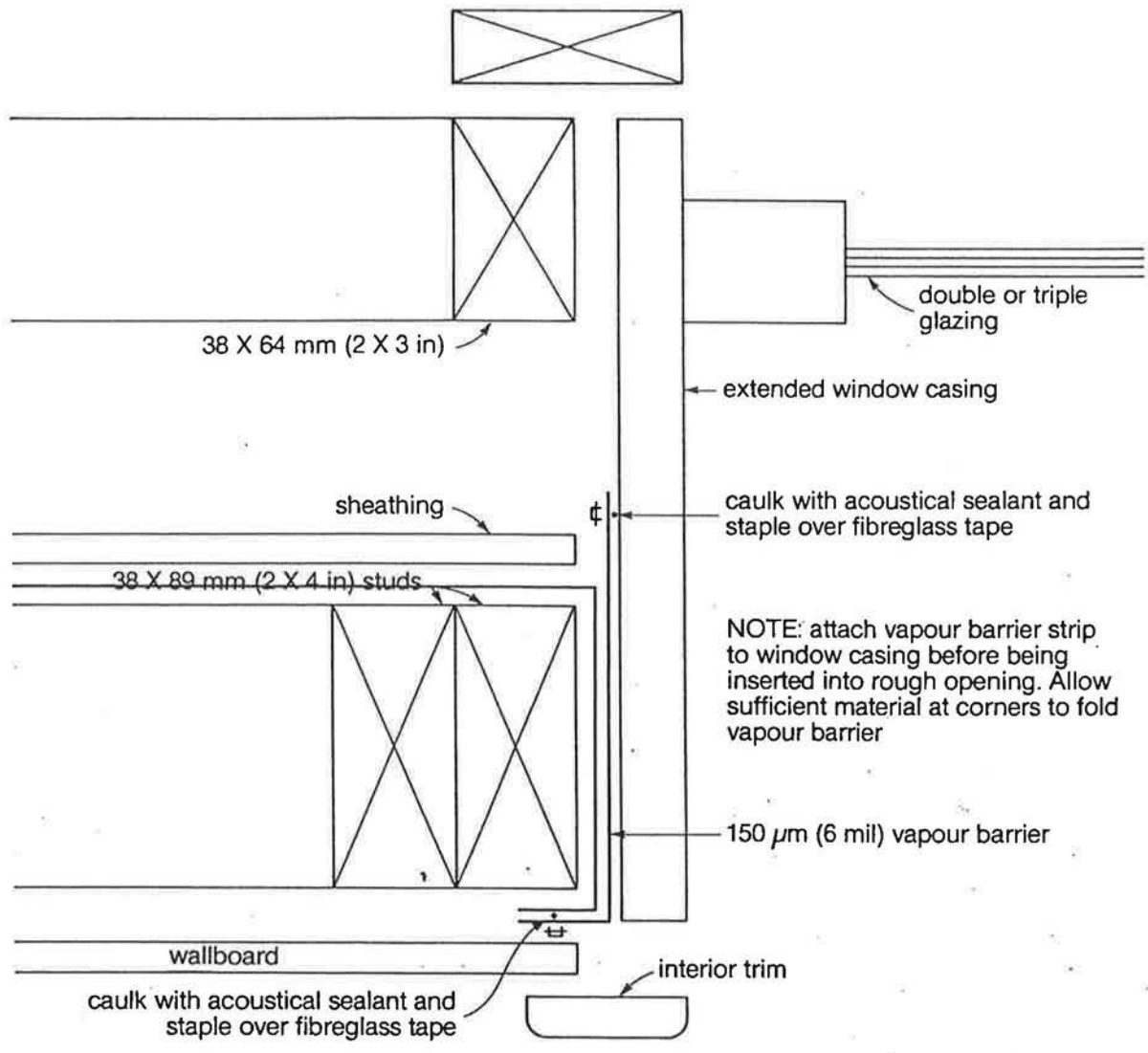
FIGURE 12. Window detail for double stud wall
