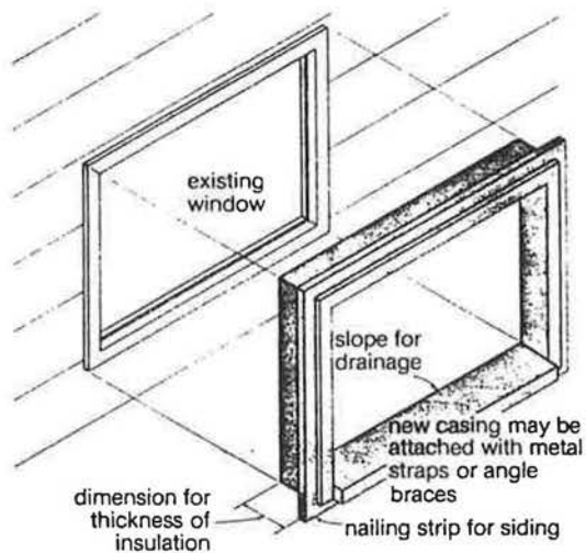
FIGURE 29. Detail of built-out window casing
