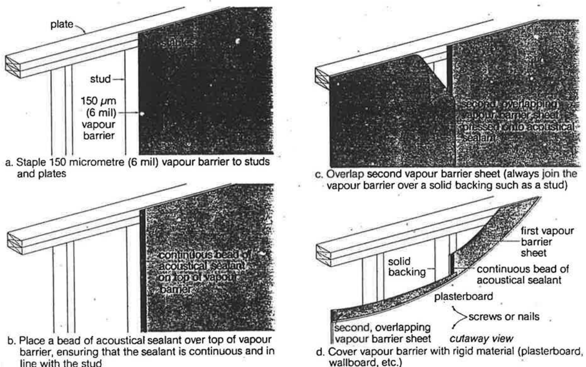
FIGURE 3. Technique for joining vapour barrier sheets on wall studs (insulation not shown)
