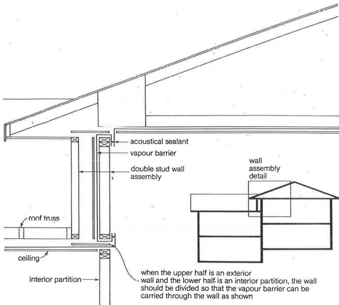
FIGURE 14. Split level house vapour barrier detail
