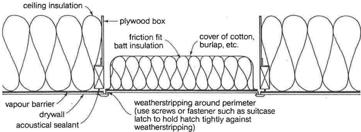
FIGURE 9. Attic hatch detail
