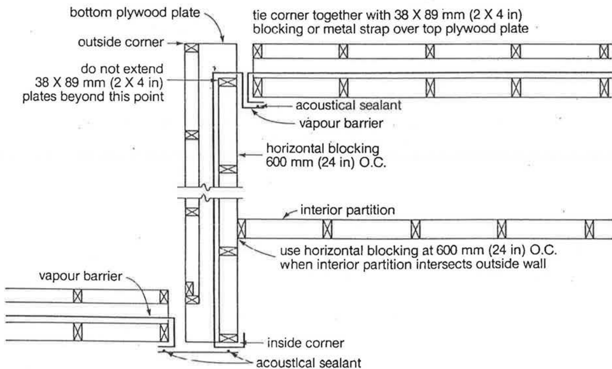
FIGURE 11. Double stud wall details
