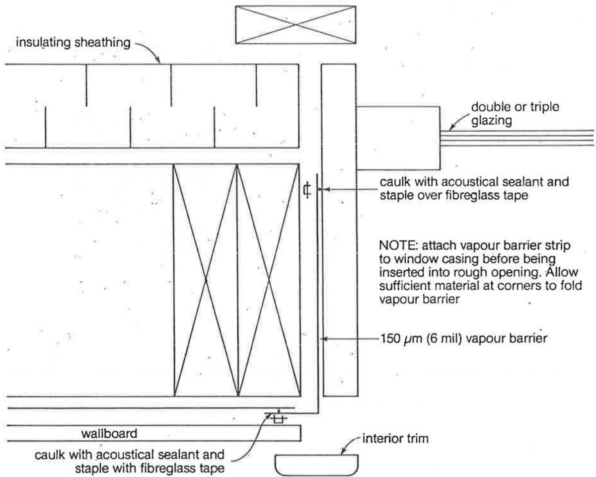
FIGURE 8. Vapour barrier installation at window
