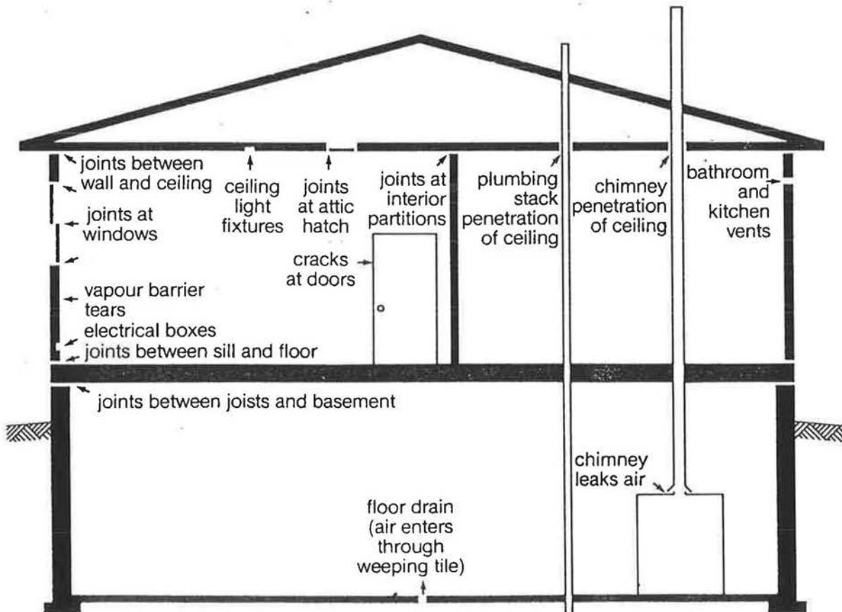
FIGURE 2. Air leakage spots in conventional housing
