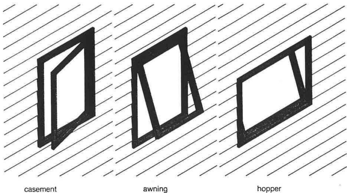
FIGURE 15. Preferred openable window types
