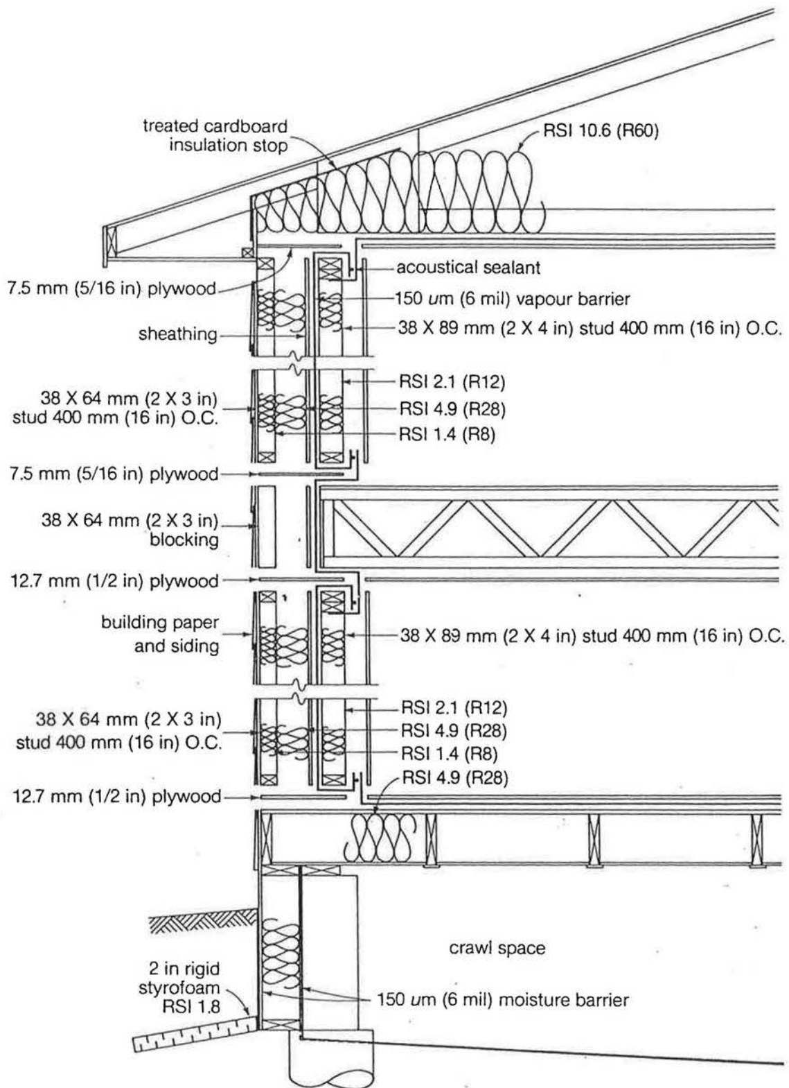
FIGURE 25. Wall section - grade beam and piling foundation
