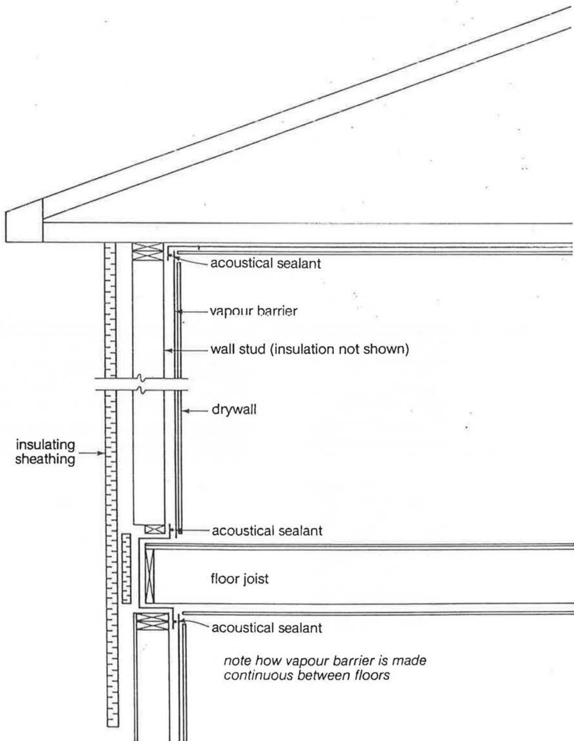
FIGURE 4. Wall section - vapour barrier detail
