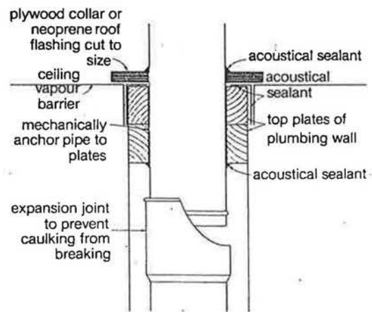
FIGURE 7. Vapour barrier installation around plumbing vent stack
