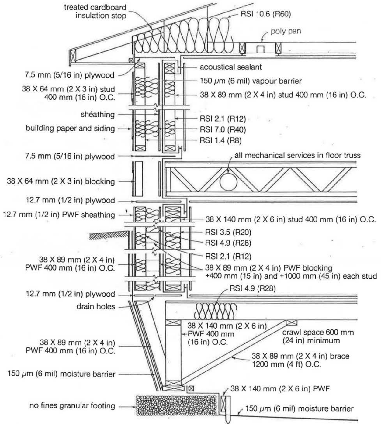
FIGURE 23. Wall section - pressure treated wood foundation
