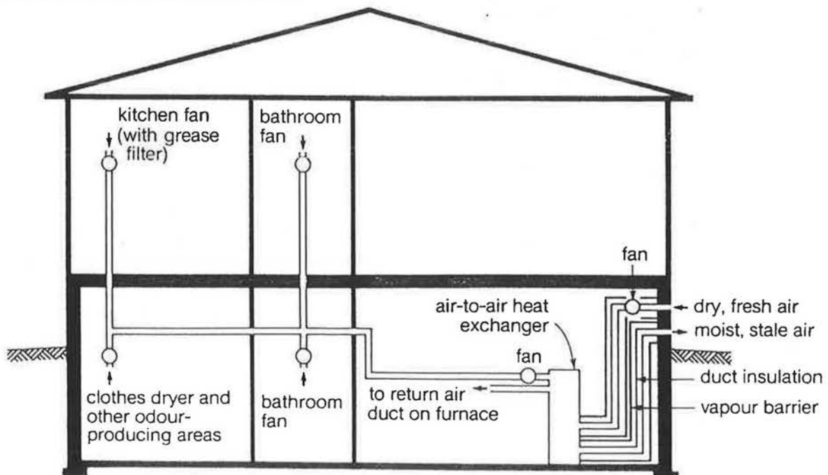
FIGURE 17. Air flow through an air-to-air heat exchanger
