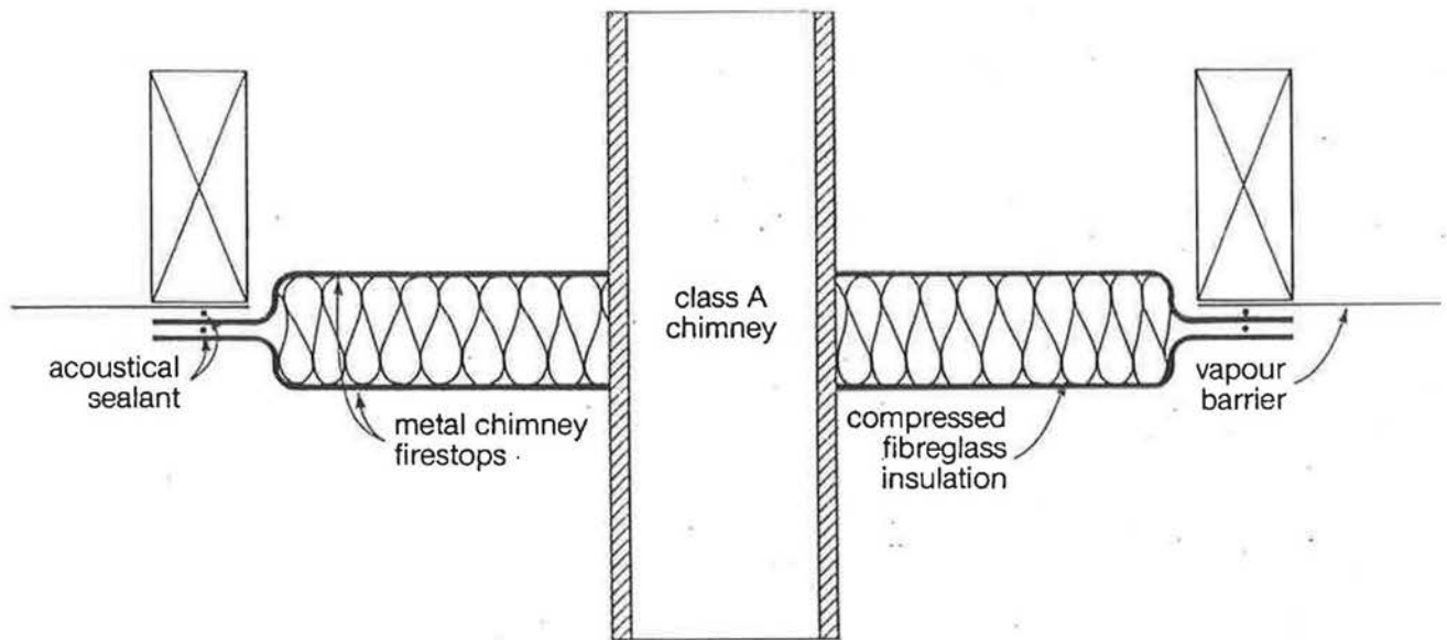
FIGURE 19. Chimney installation detail
