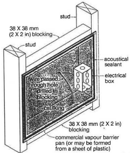
FIGURE 6. Vapour barrier installation around electrical box
