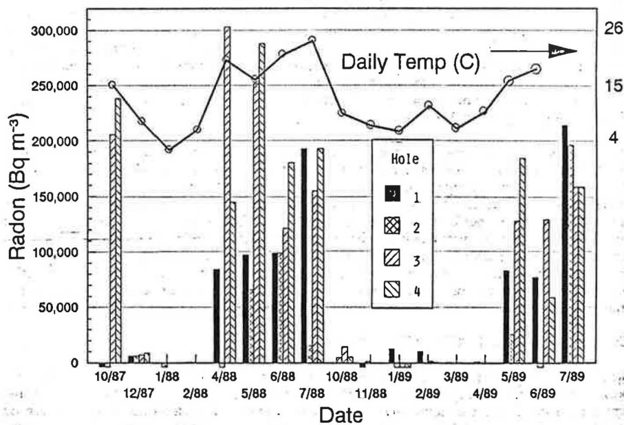
Fig. 1. Grab samples measurements by Lucas cell of radon in air from four natural holes in the backyard of Huntsville house; negative values indicate that no measurement was made at a particular hole. The mean daily outdoor temperature is indicated for days that the holes were sampled.
