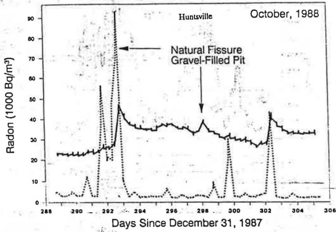
Fig. 2. Radon issuing from natural hole 1 and within a 1 m deep, gravel-filled, clay-capped pit, 8 m distance from hole 1.
