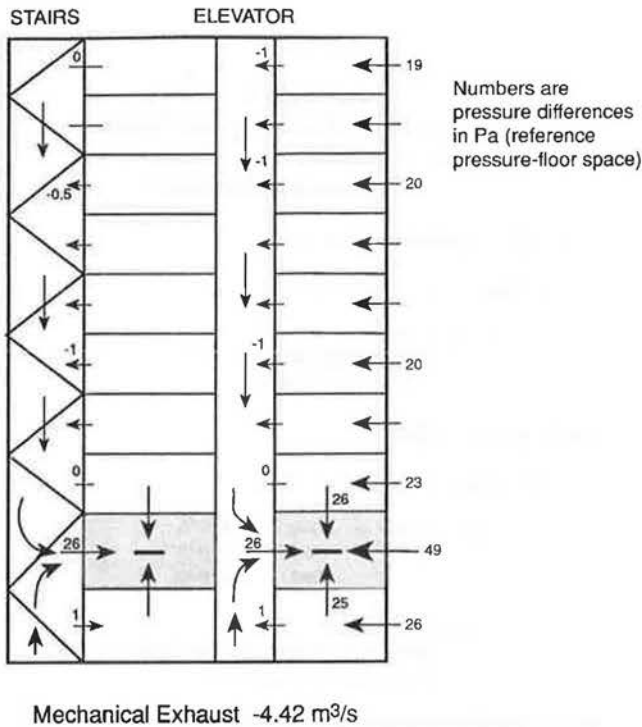
Figure 3 Airflow and pressure difference patterns caused by mechanical smoke exhaust system (MSES)—nonfire.
