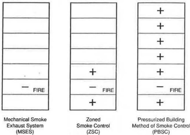
Figure 2 Description of test smoke control systems.
