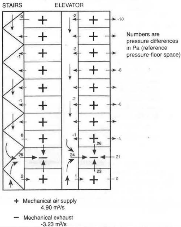
Figure 5 Airflow pressure difference patterns caused by pressurized building method of smoke control (PBSC)—nonfire.
