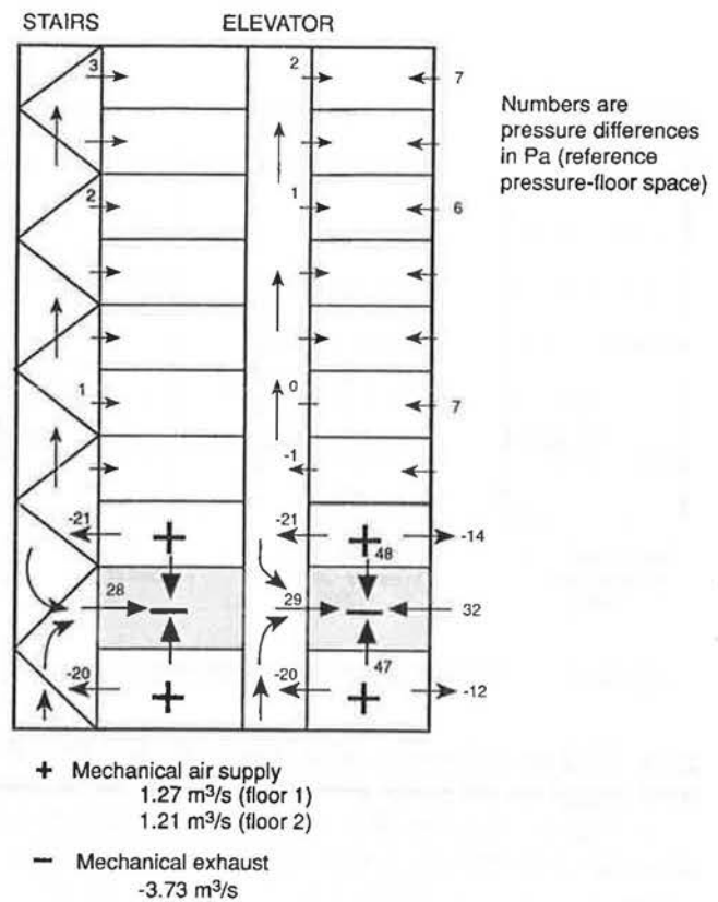
Figure 4 Airflow and pressure difference patterns caused by zoned smoke control (ZSC)—nonfire.
