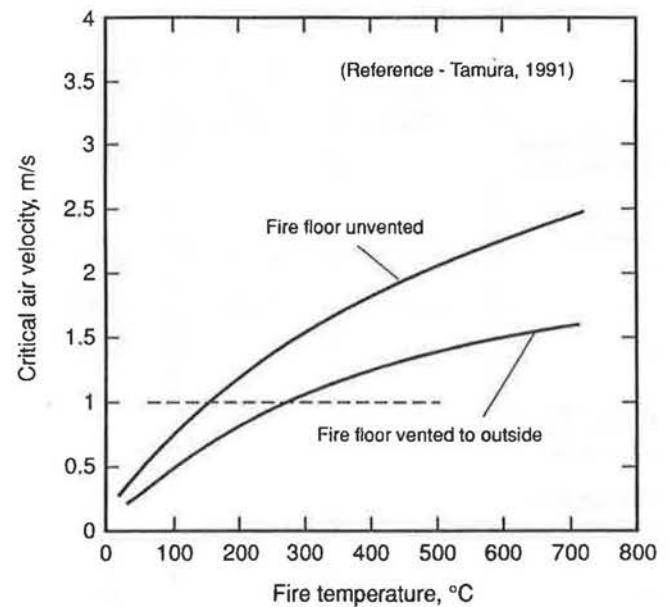
Figure 6 Critical air velocity vs. fire temperature.
