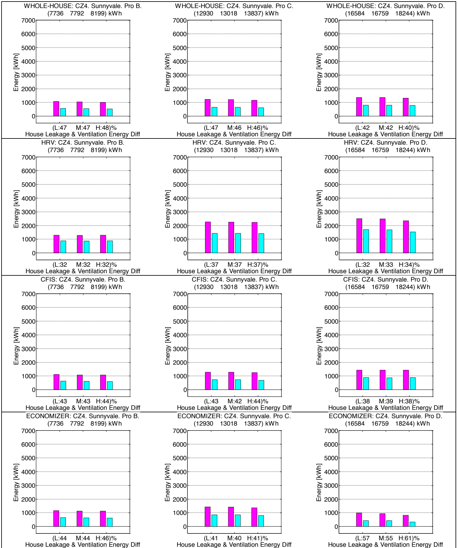
Figure 32: Ventilation-related energy penalty with and without RIVEC for climate zone 4, Sunnyvale
