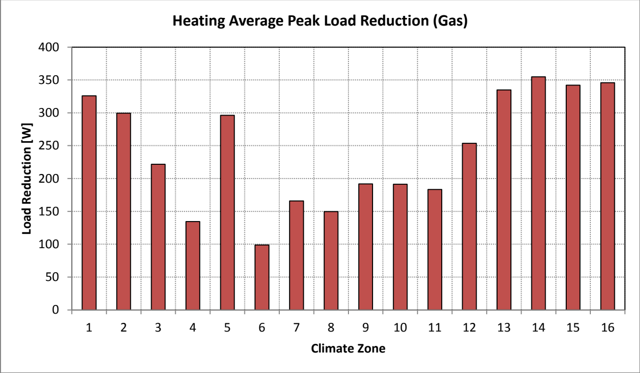
Figure 28: Heating average peak load reduction over the year from using RIVEC (whole-house exhaust, Prototype C, medium leakage)
