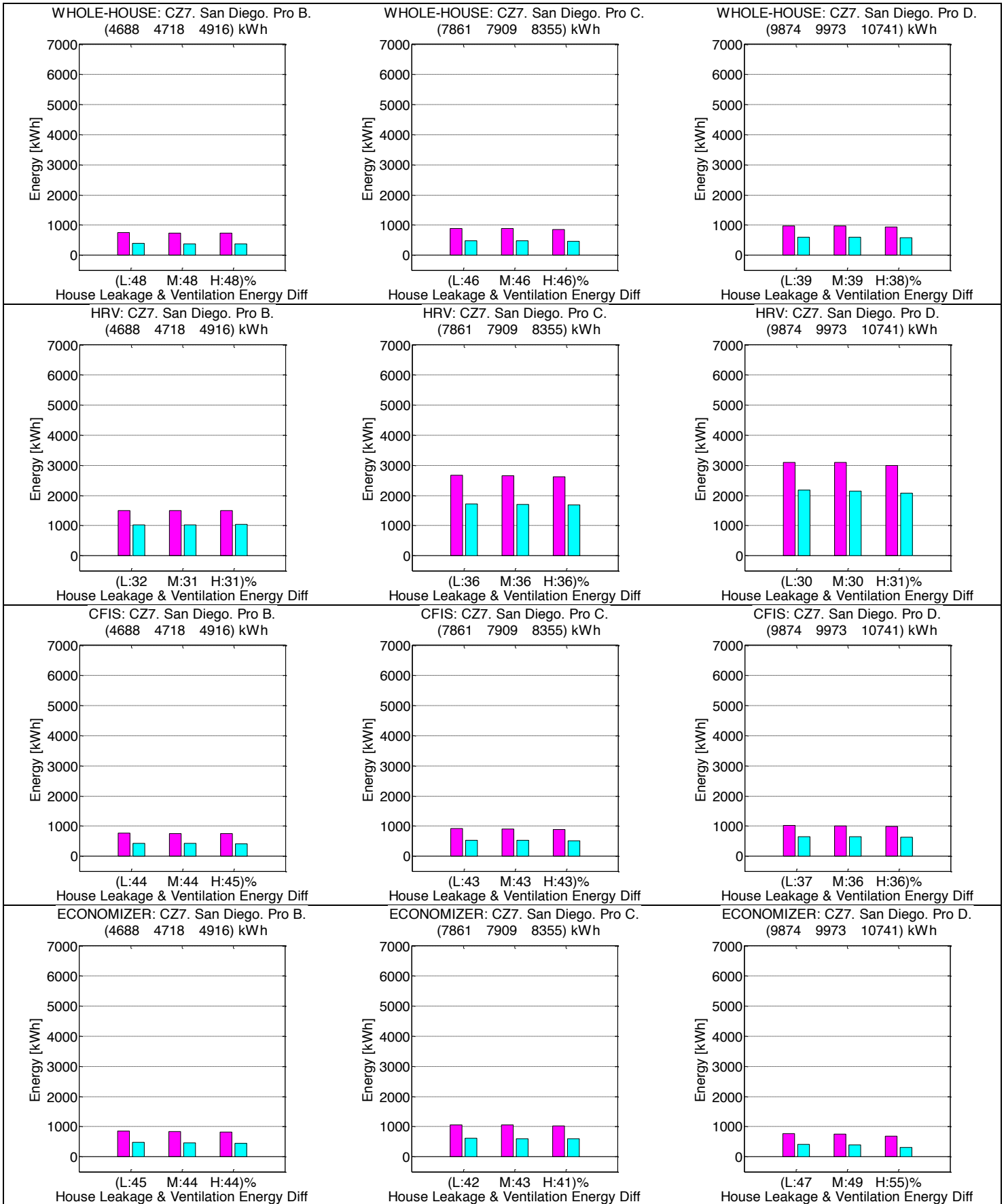
Figure 35: Ventilation-related energy penalty with and without RIVEC for climate zone 7, San Diego
